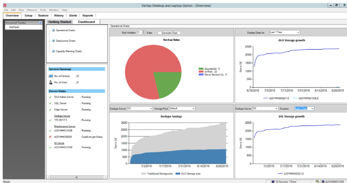
Figure 2-3 DLO Dashboard
